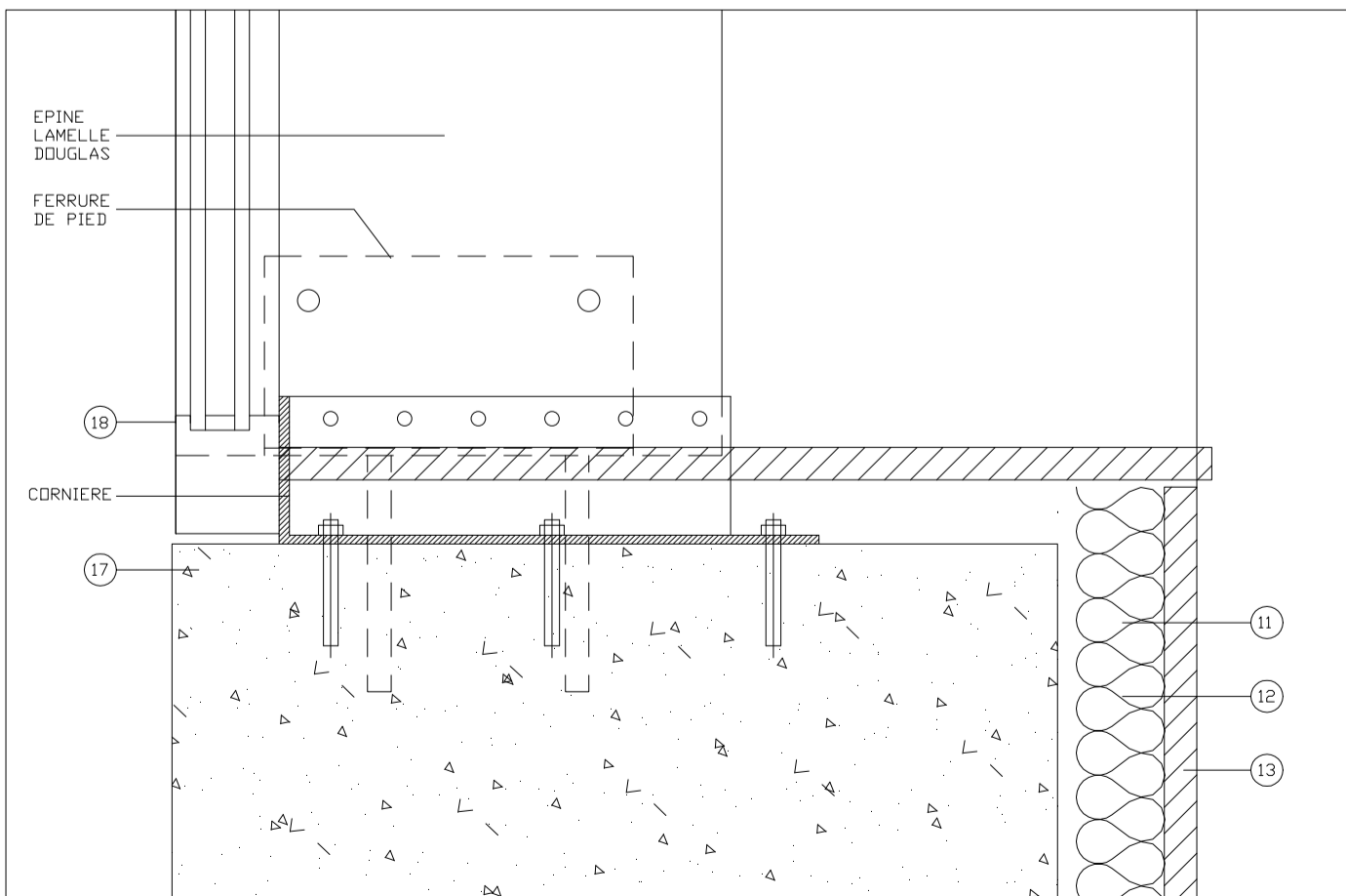
DETAIL 6 1_5
