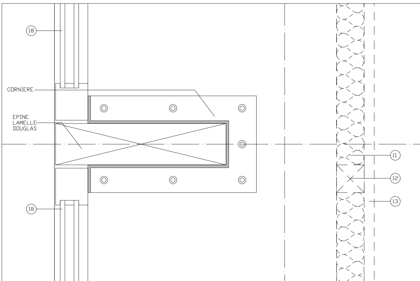
DETAIL 5 1_5
