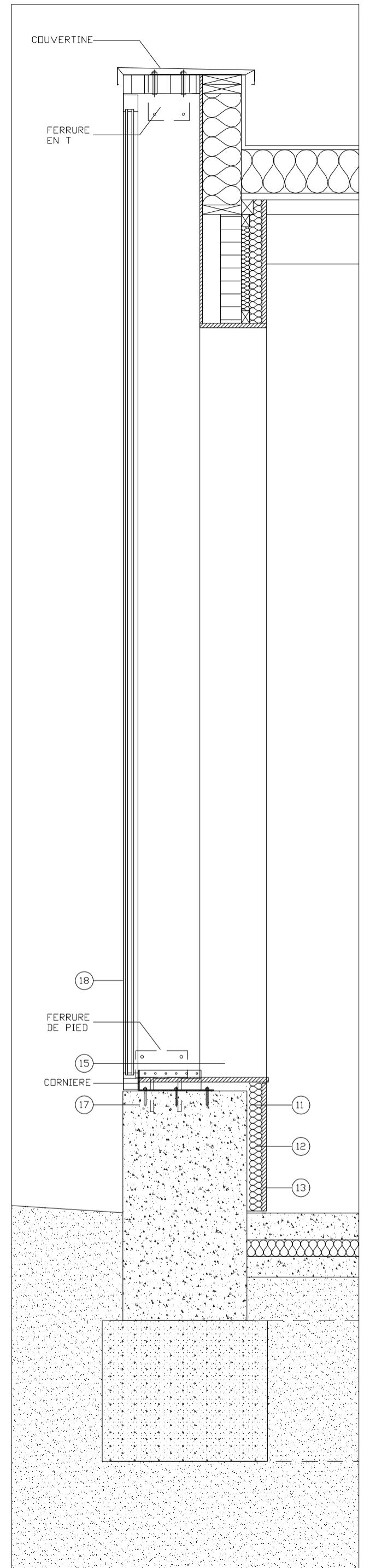
COUPE E 1_20
