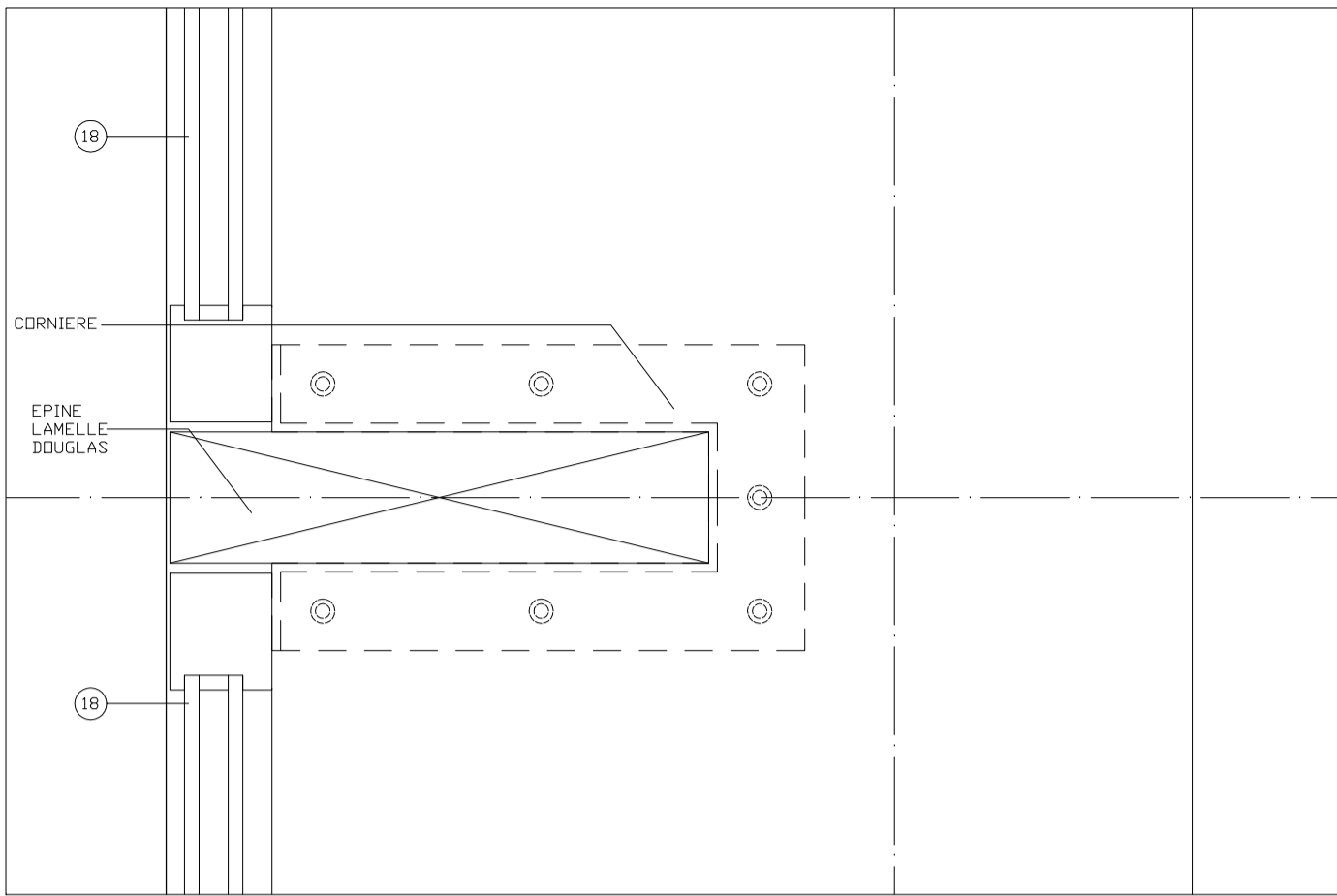
DETAIL 4 1_5
