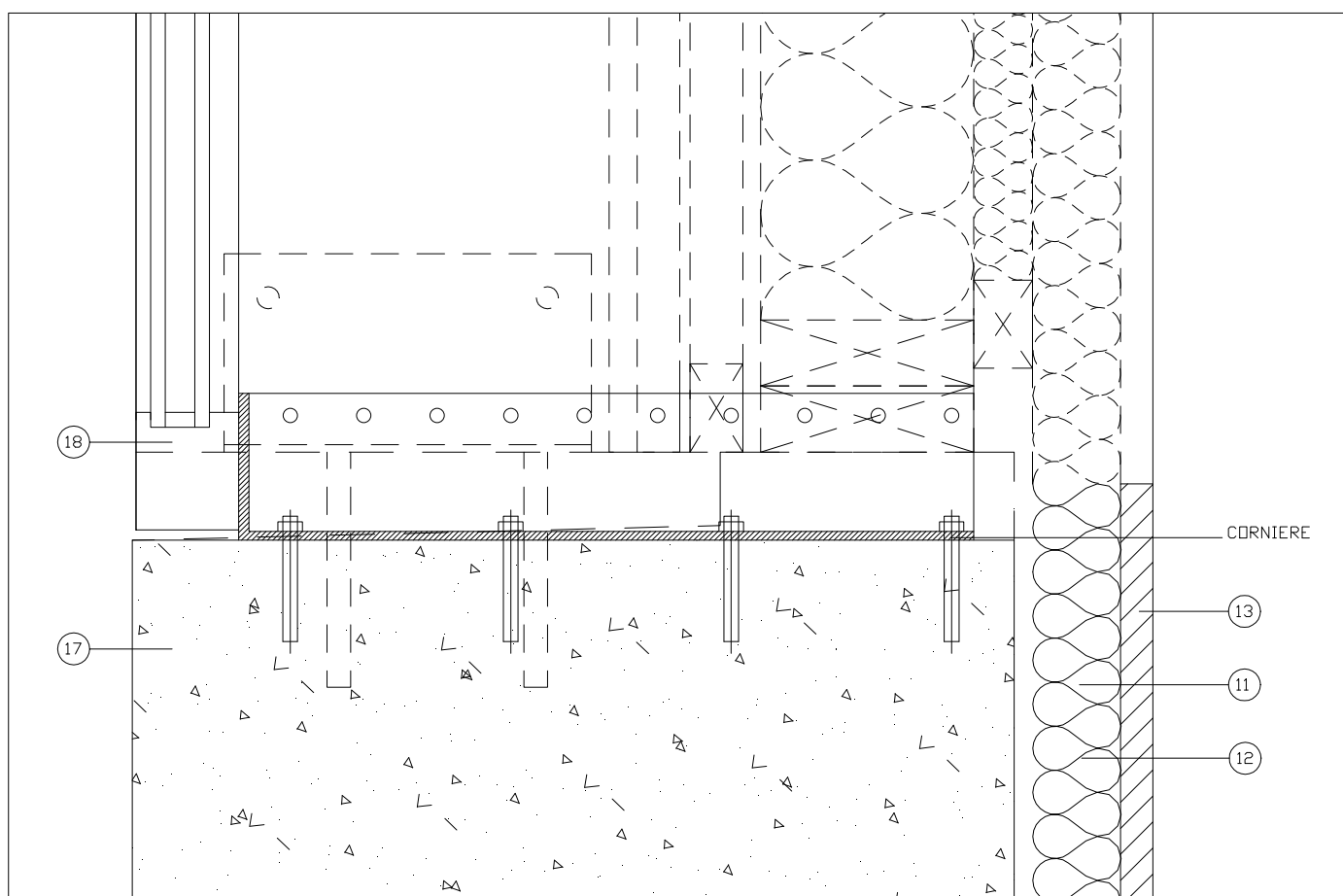
DETAIL 3 1_5
