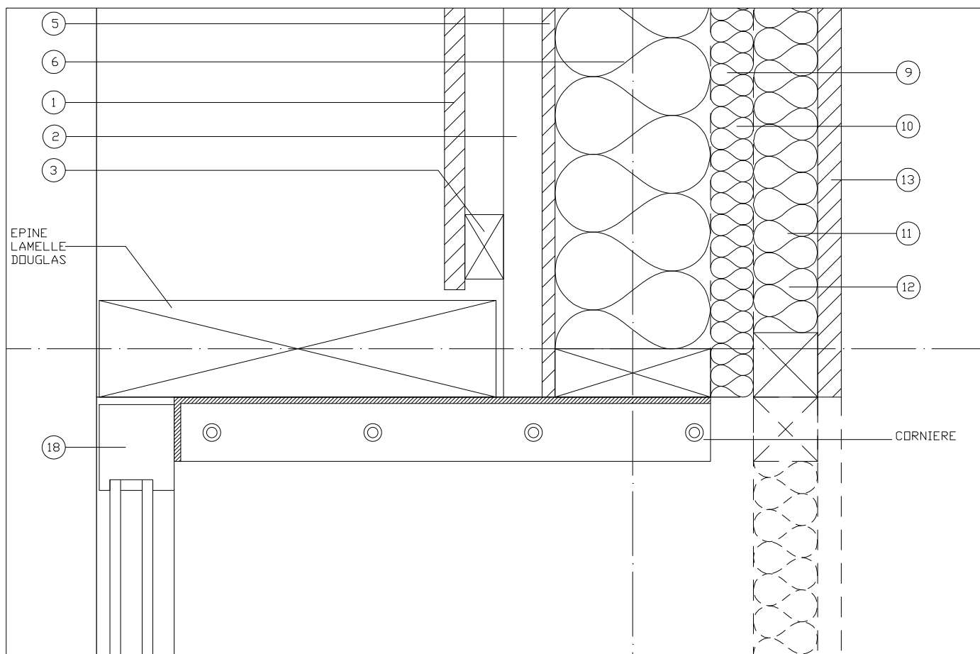
DETAIL 2 1_5
