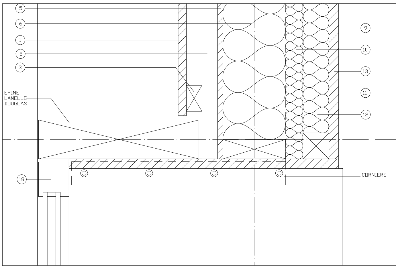
DETAIL 1 1_5
