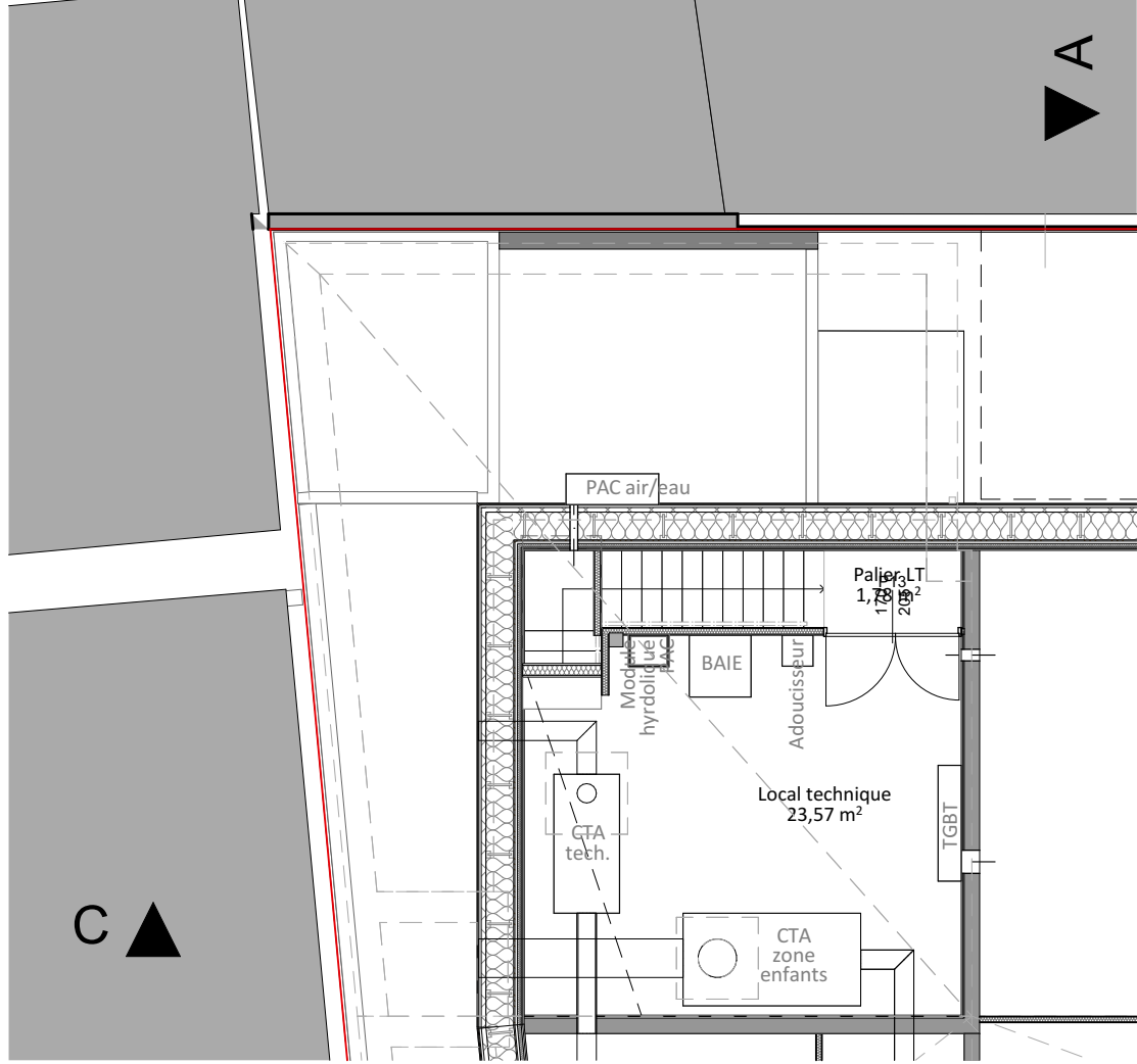
Plan R+1
