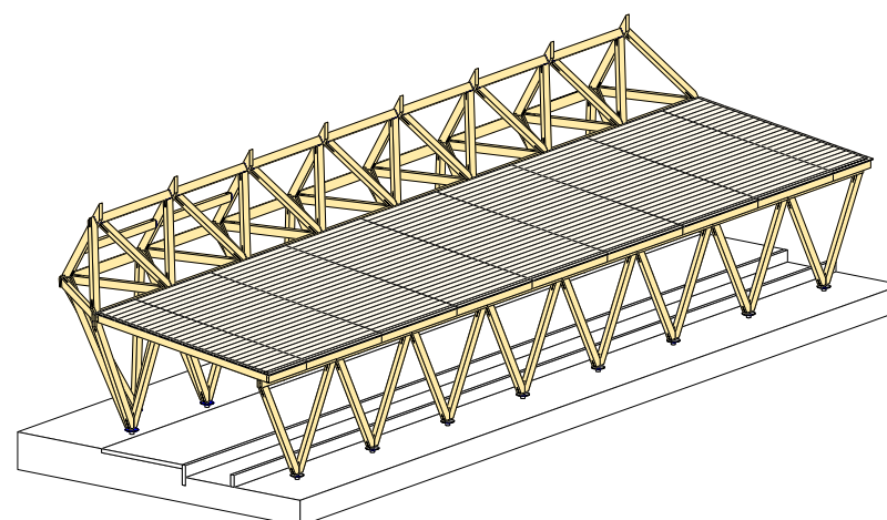
LEVAGE TRIPODES - ensemble parties hautes
