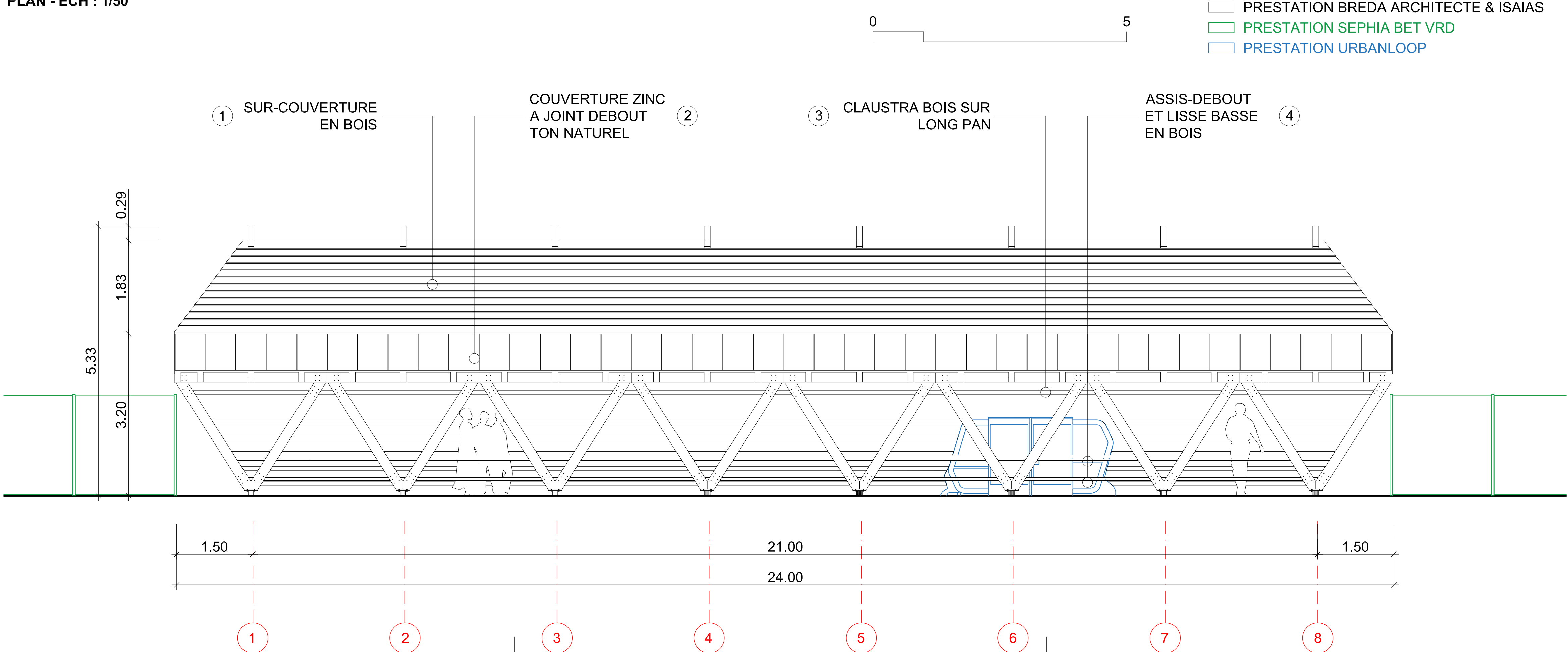
ELEVATION - ECH : 1/50
