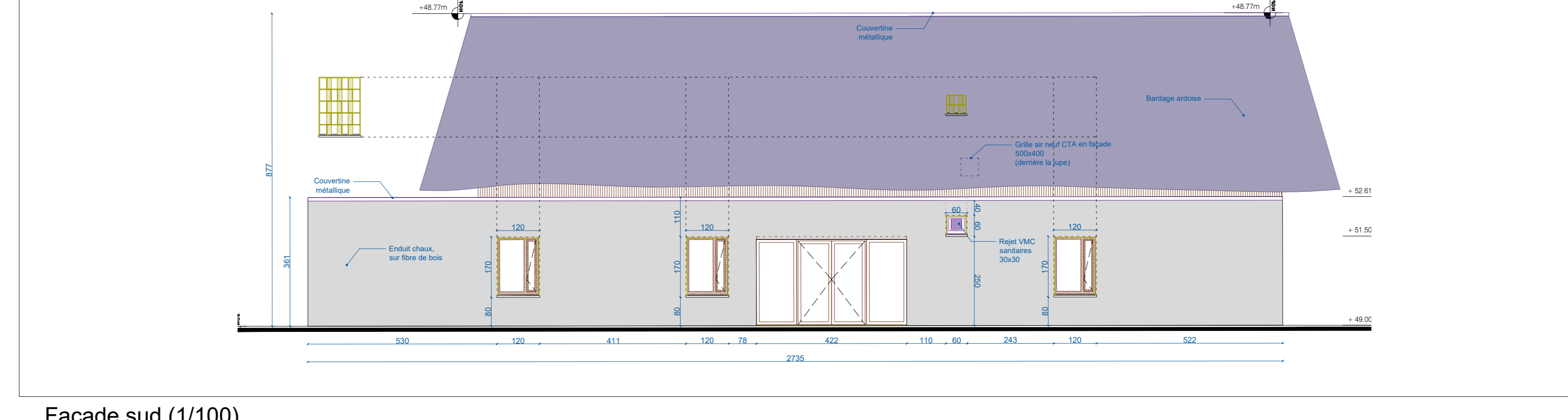
Façade sud (1/100)
