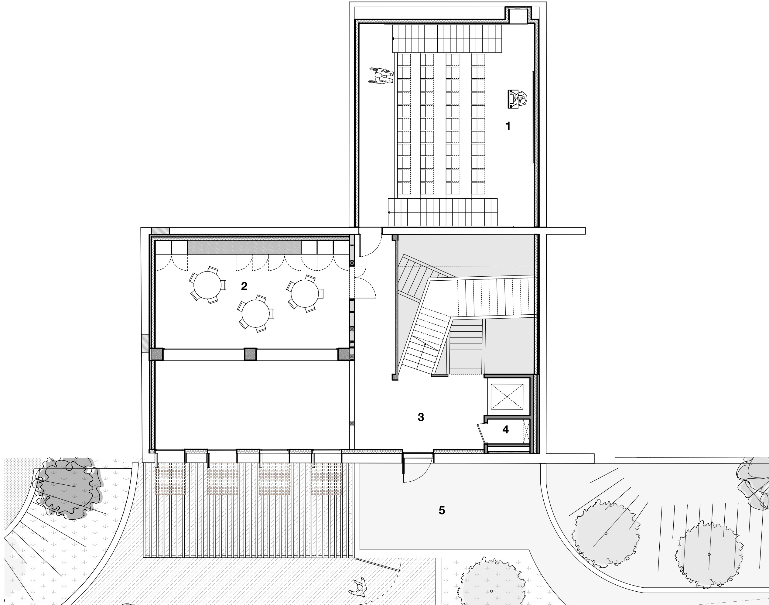
PLAN R-1
