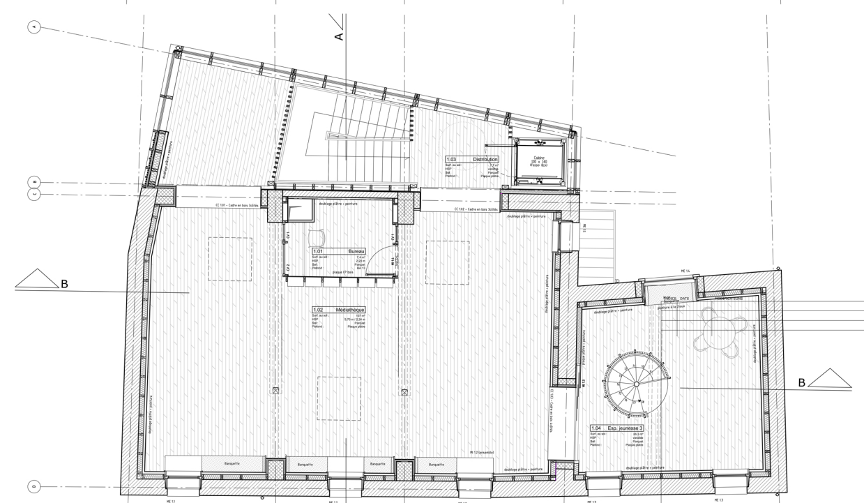
PLAN R+1 Echelle 1/50
