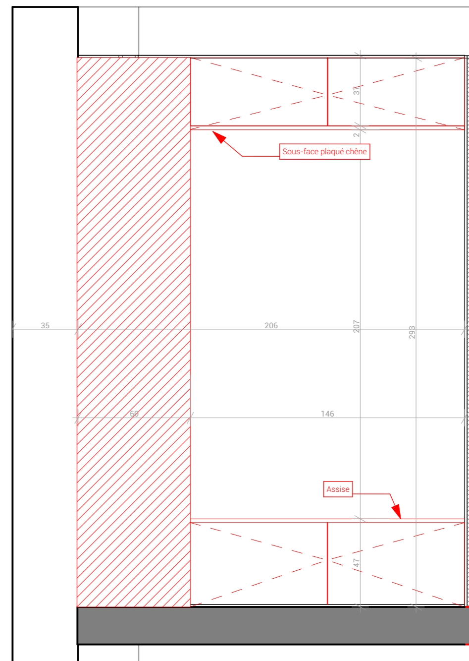
ELEVATION MEUBLE 2
