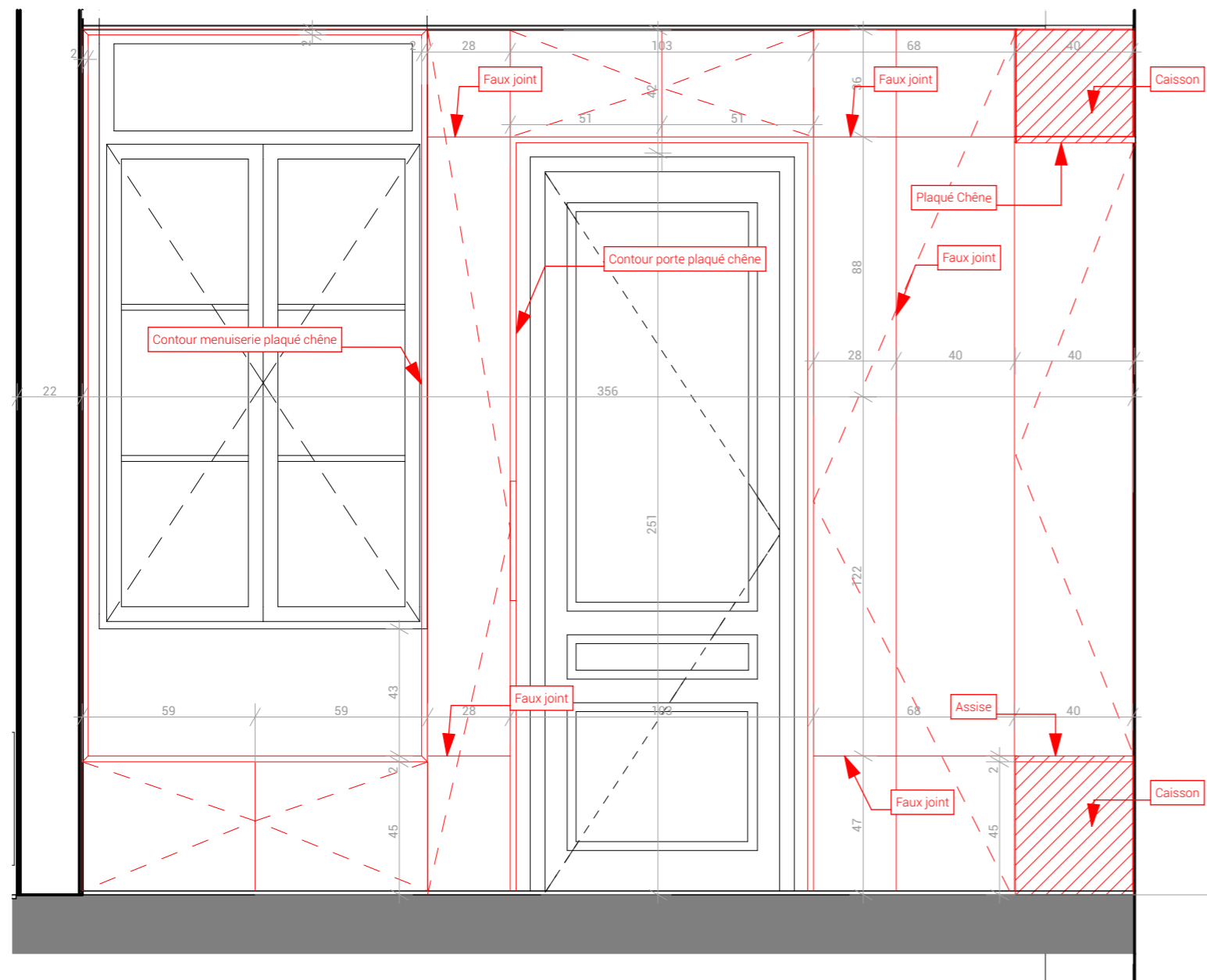
ELEVATION MEUBLE 1
