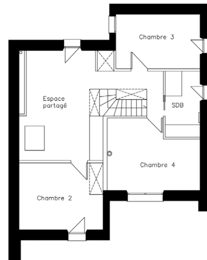
Plan r+1
