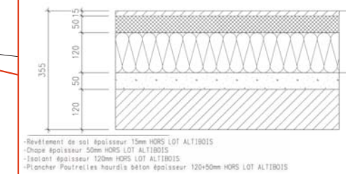
PB / Complexe DALLAGE
