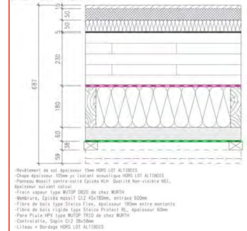
M1 / Complexe MUR Bardage
