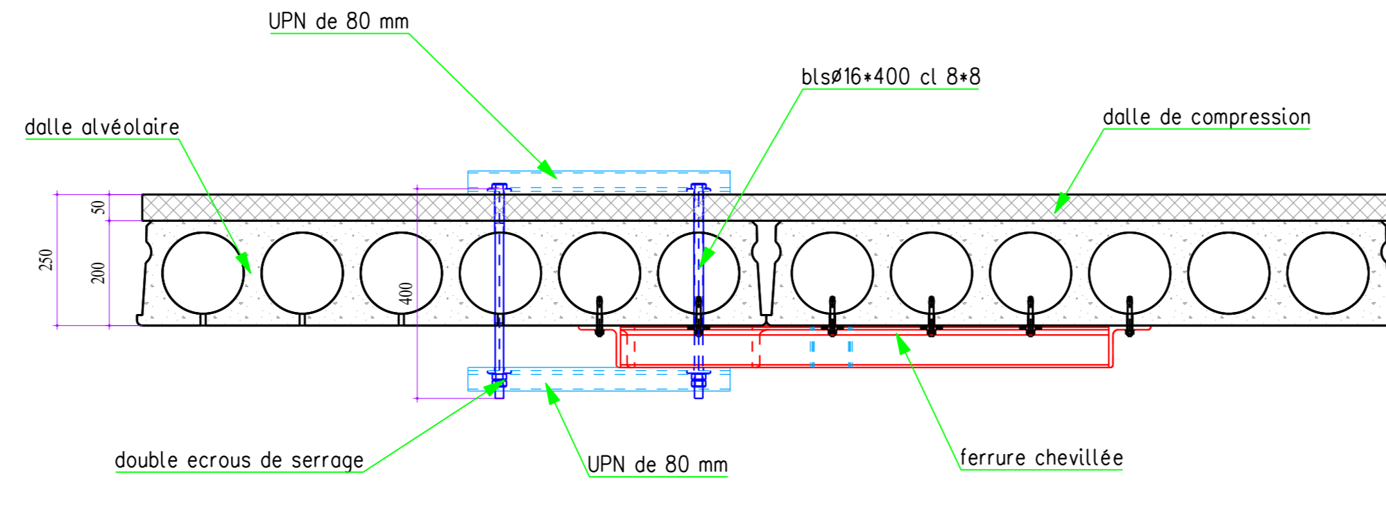
DETAIL FIXATION
