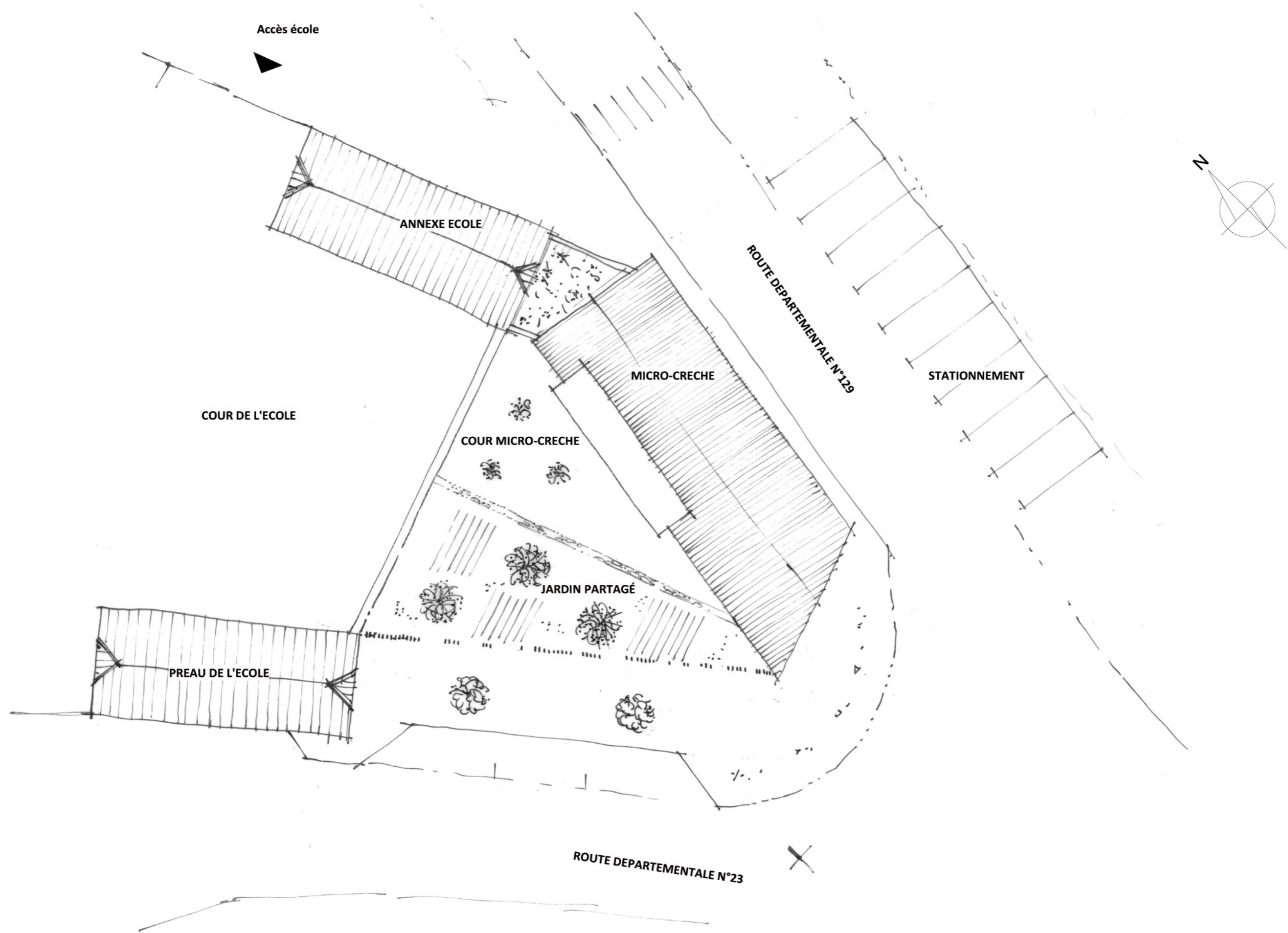
PLAN-MASSE - Ech: 1/200
