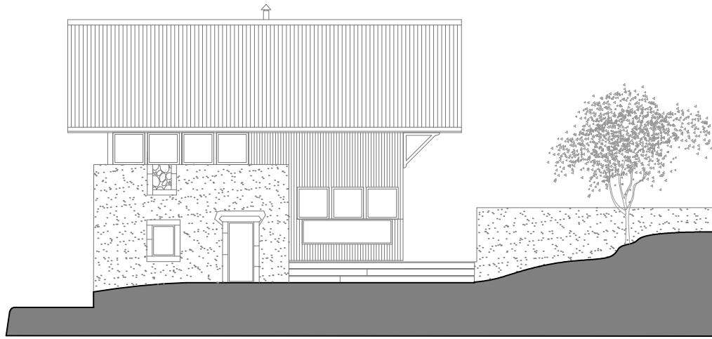
FACADE SUD
