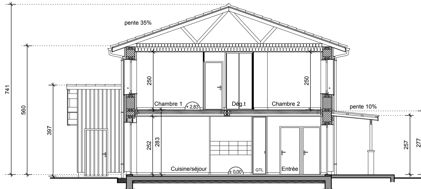
COUPE AA (log.t 4)
