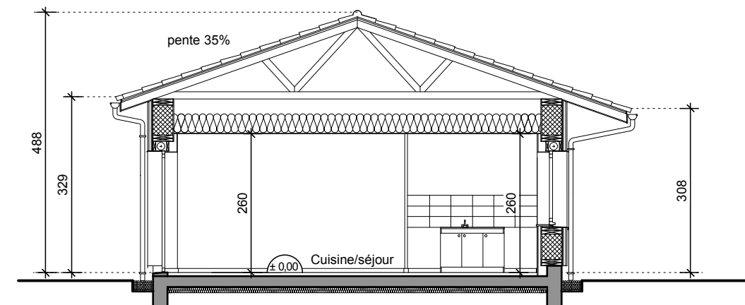
COUPE CC (log.t 11)
