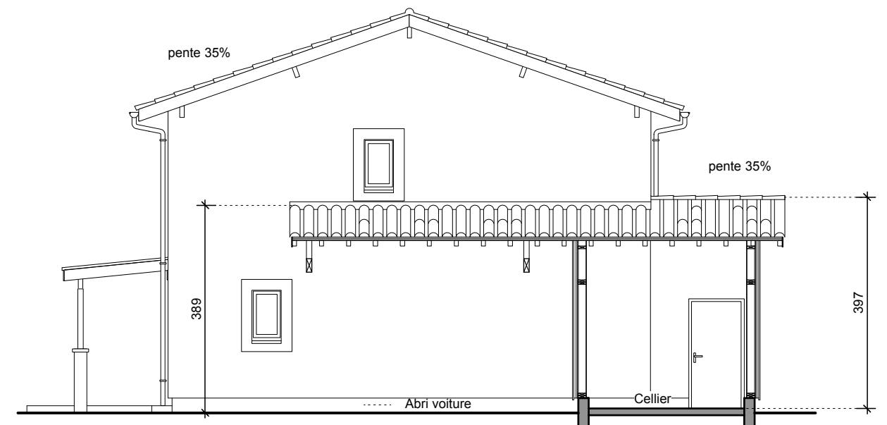
COUPE BB (log.t 4)
