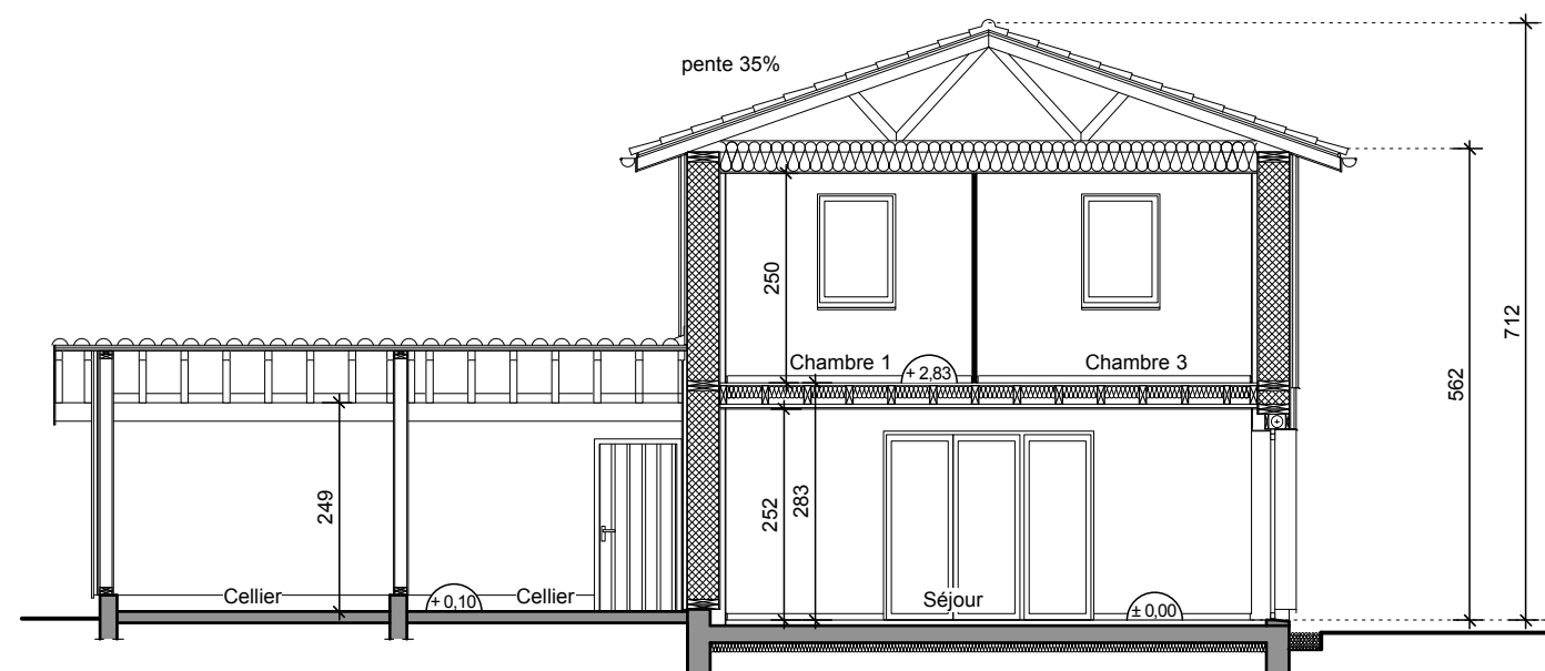
COUPE CC (log.t 7)
