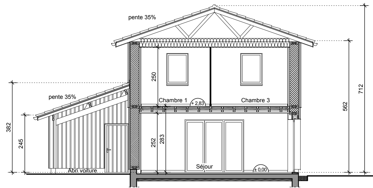
COUPE AA (log.t 8)
