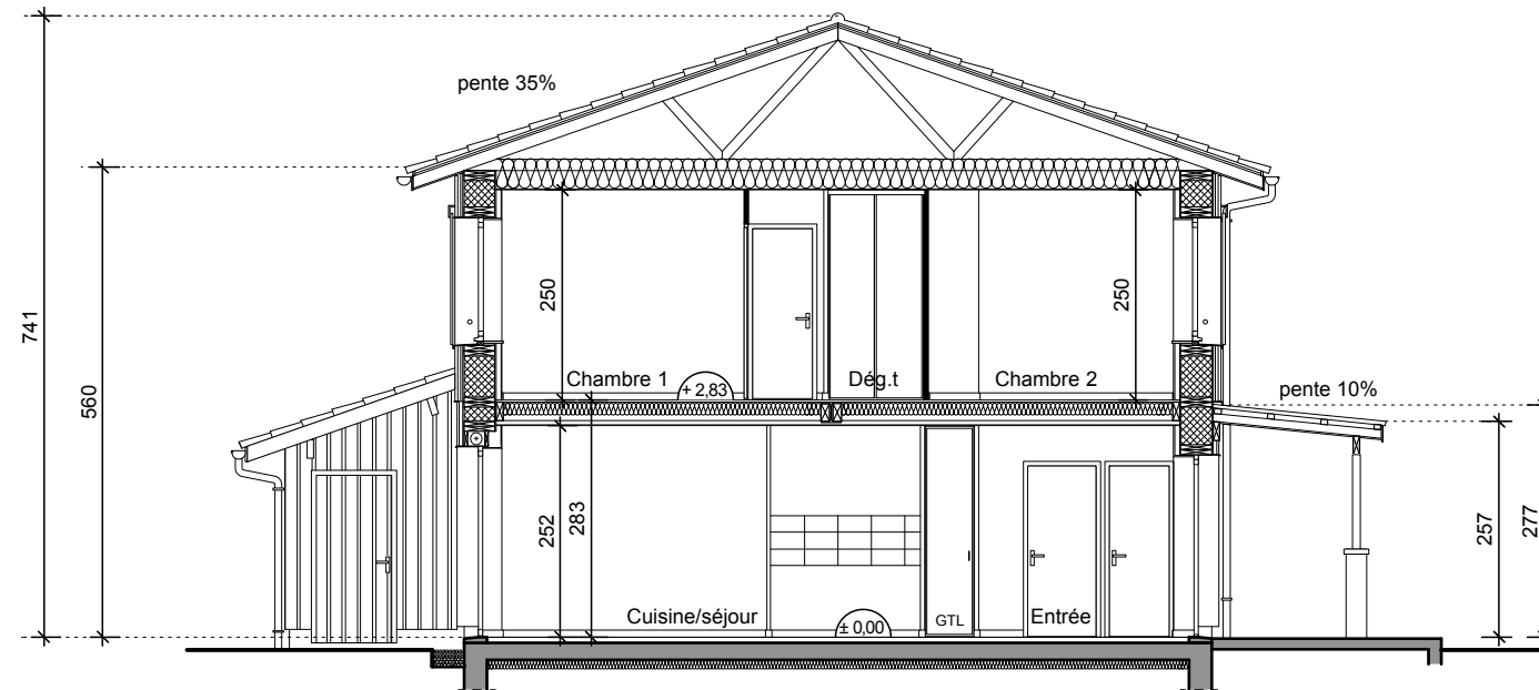
COUPE AA (log.t 2)
