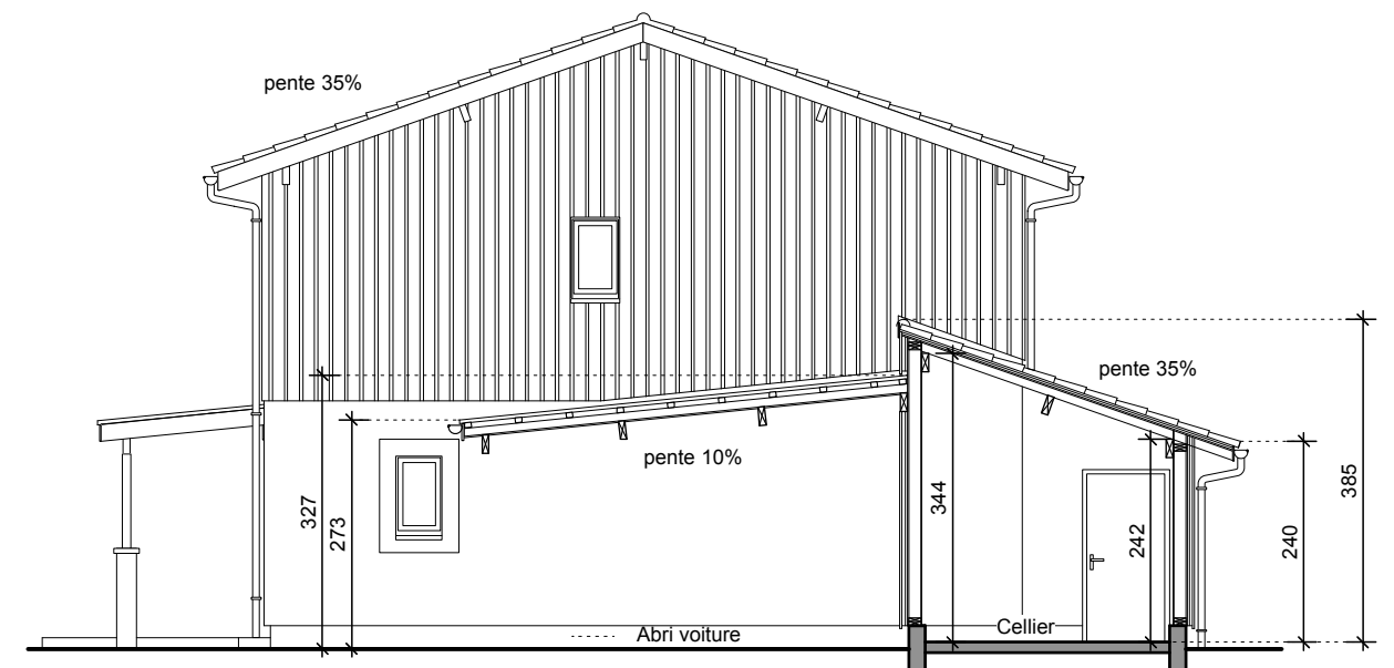
COUPE BB (log.t 2)
