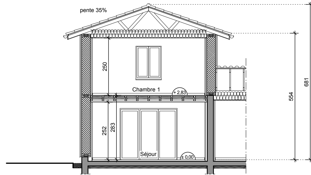
COUPE AA (log.t 9)
