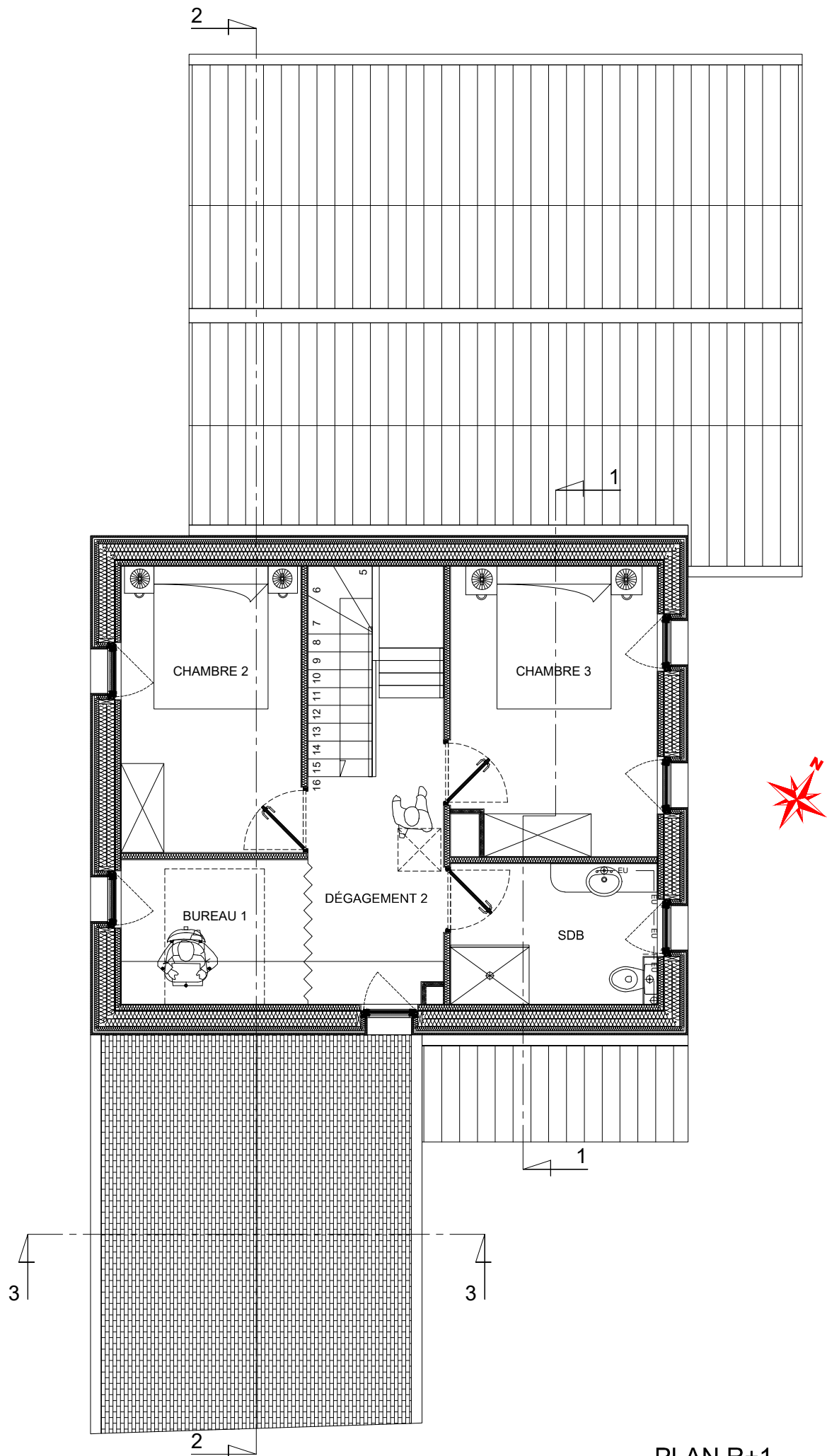
PLAN R+1
