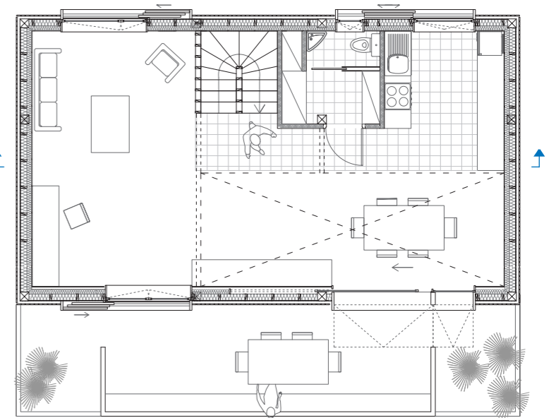
PLAN R+1
