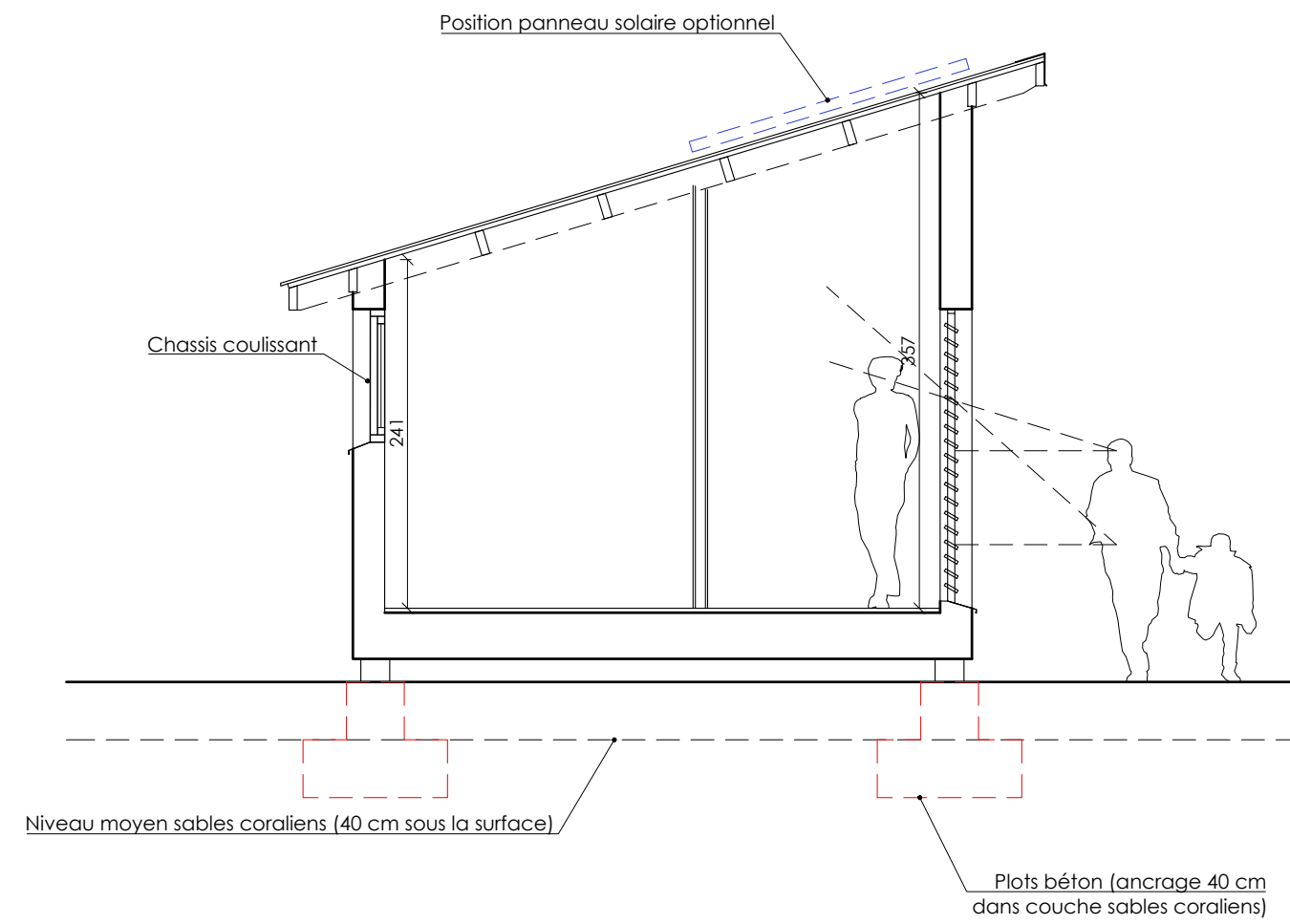
COUPE AA HLL DOUBLE PMR CLIMATISE
