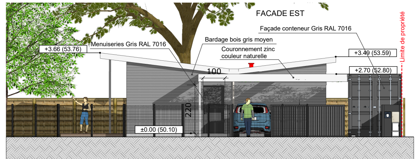
PLAN FACADES
