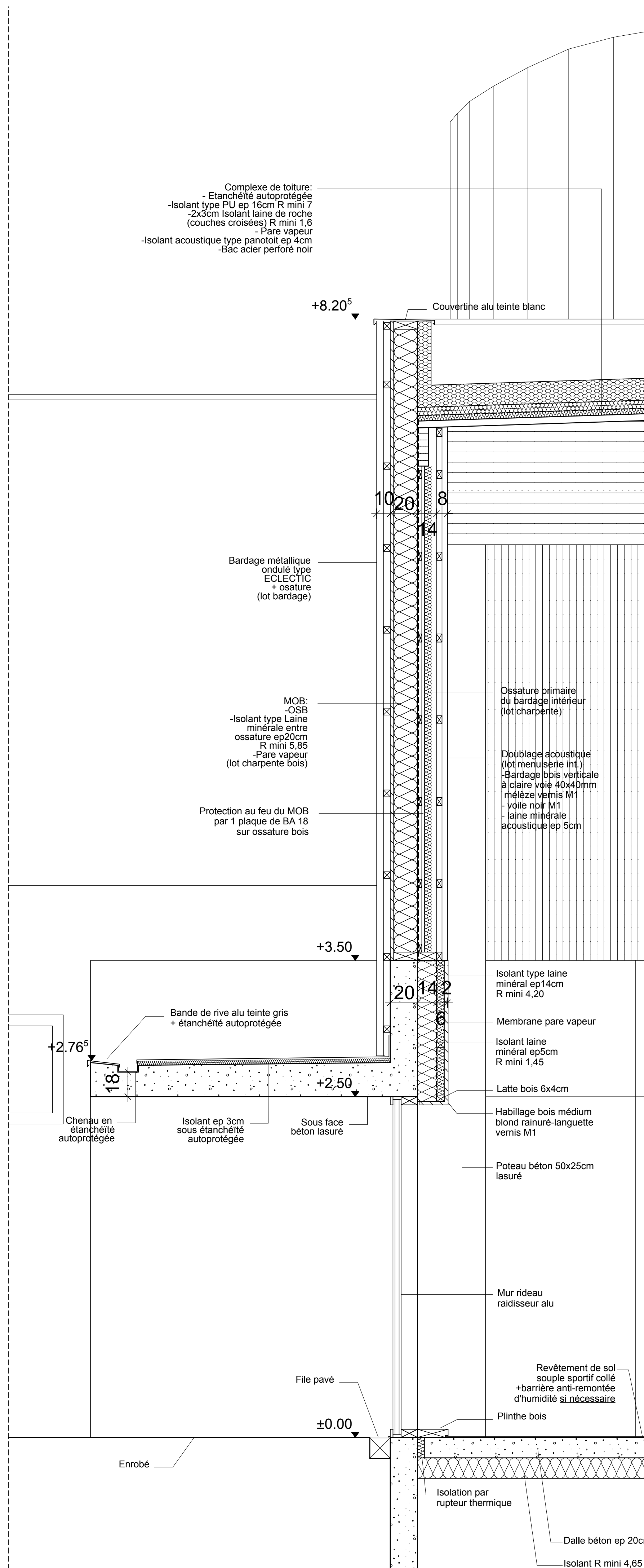
COUPE DETAIL 1 FACADE EST EXTENSION
