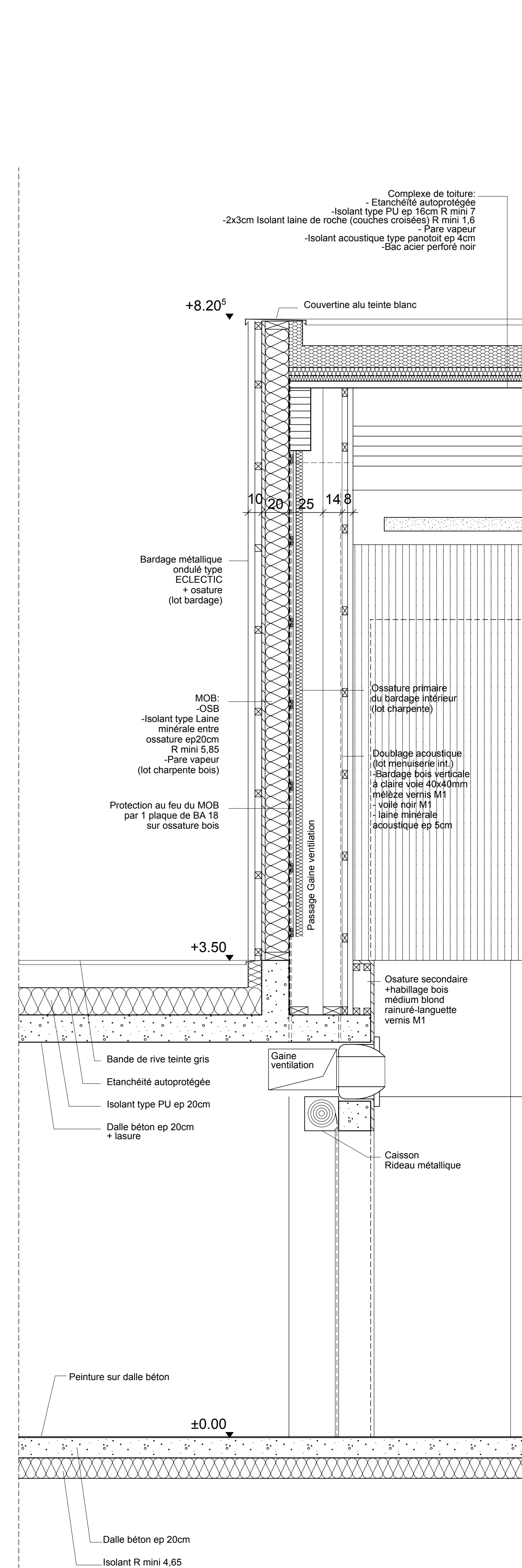
COUPE DETAIL 3 FACADE SUD EXTENSION
