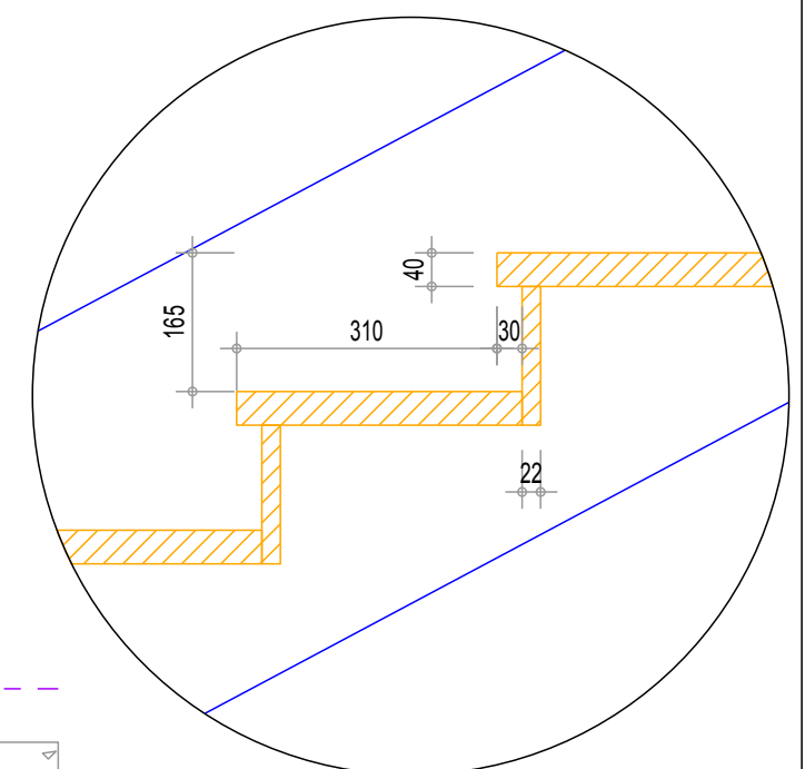
DETAIL B
