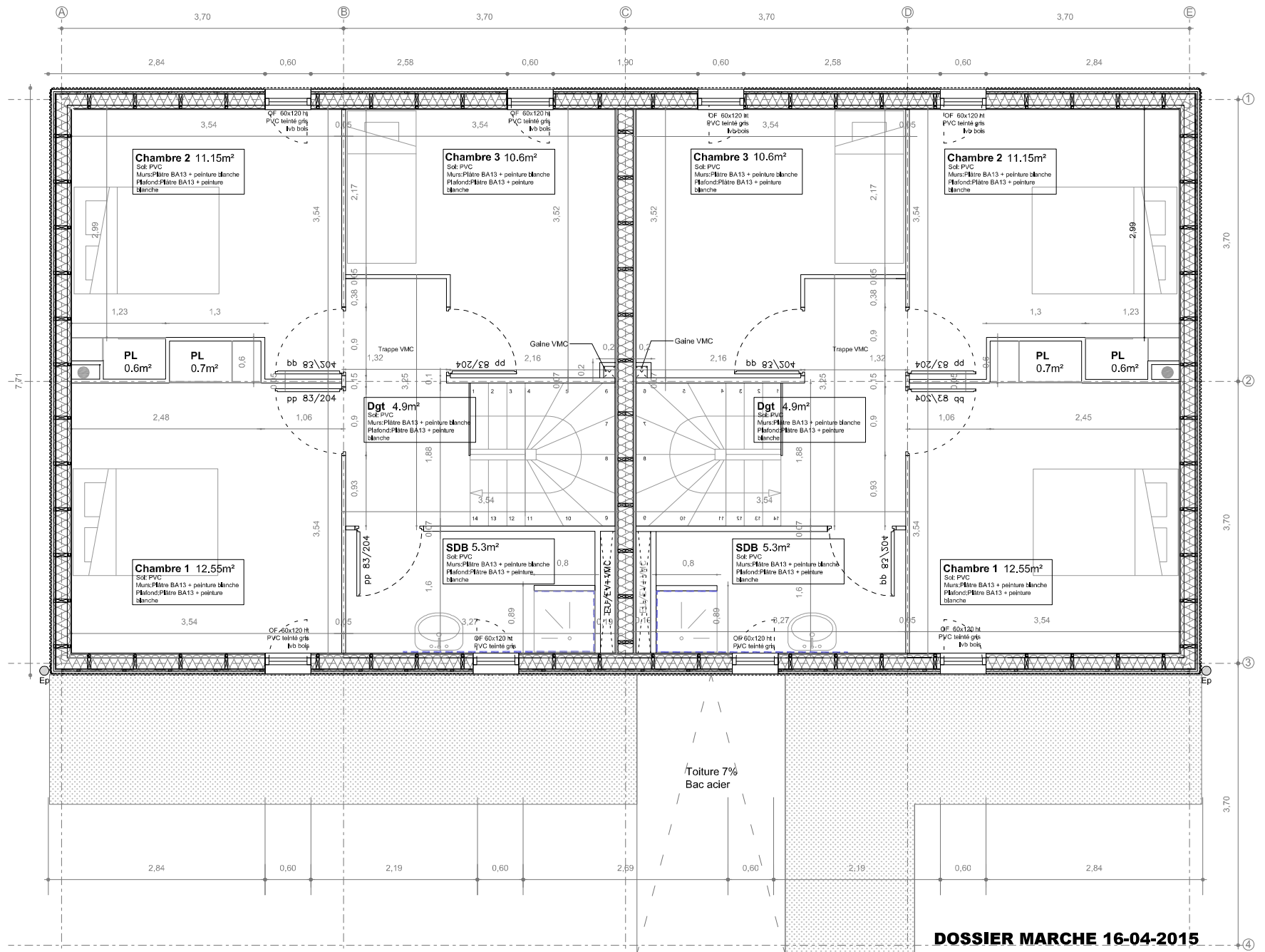
Plan R+1
