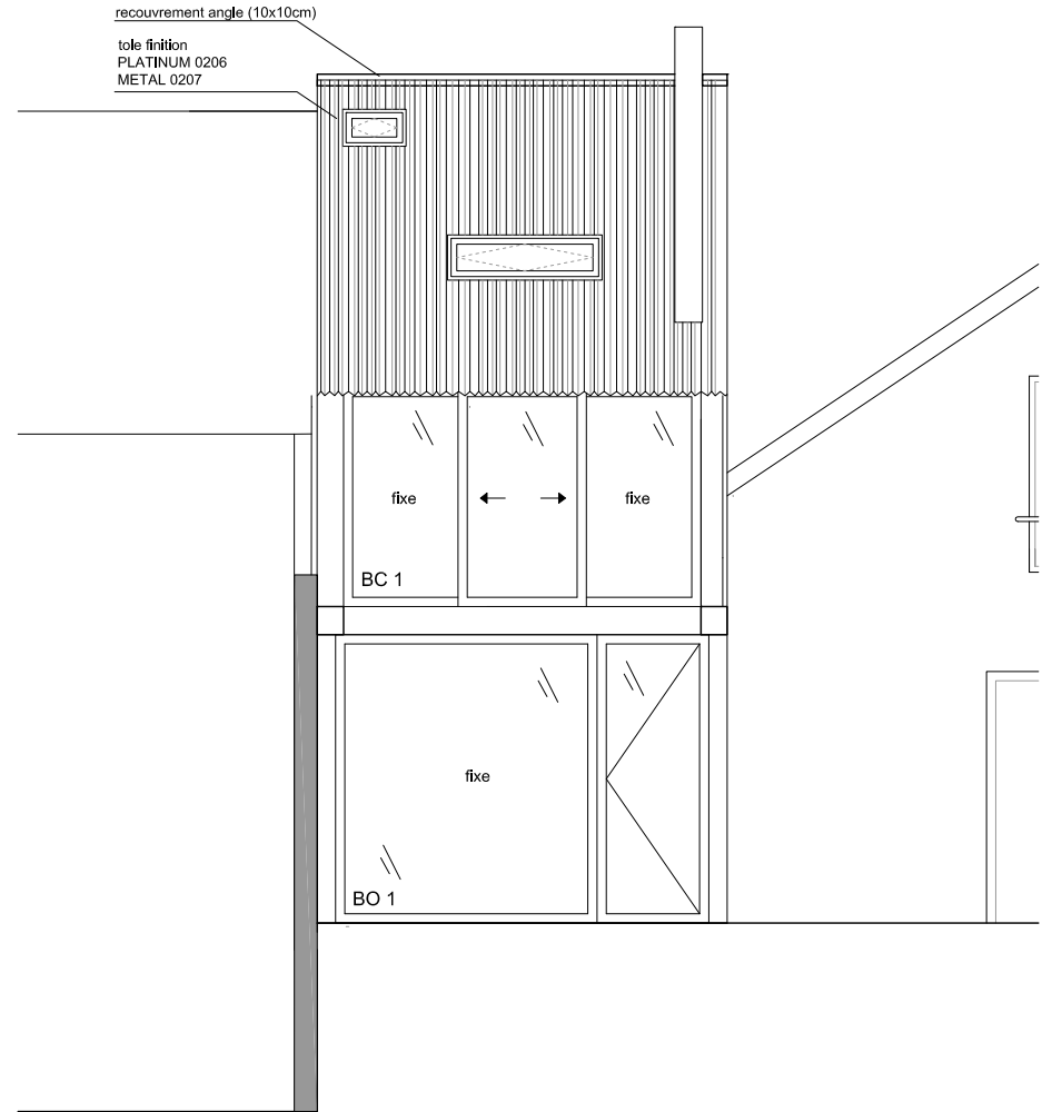
FACADE SUD
