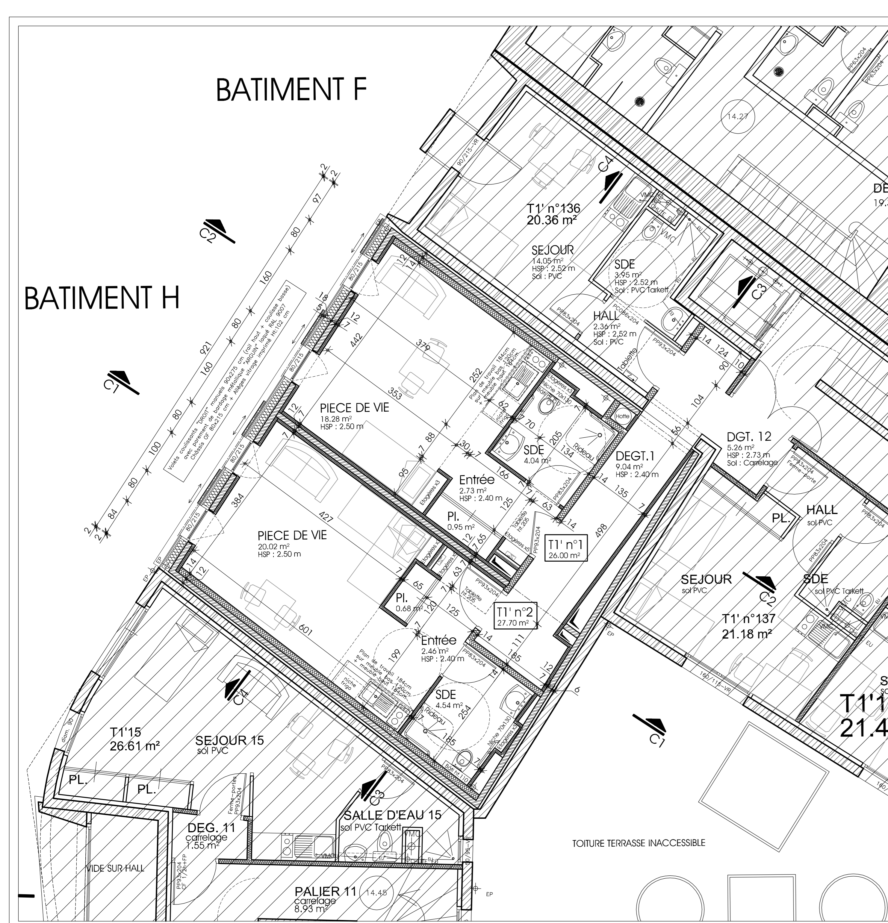
PLAN ETAGE 1 - 1/50
