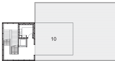
PLAN R+1
