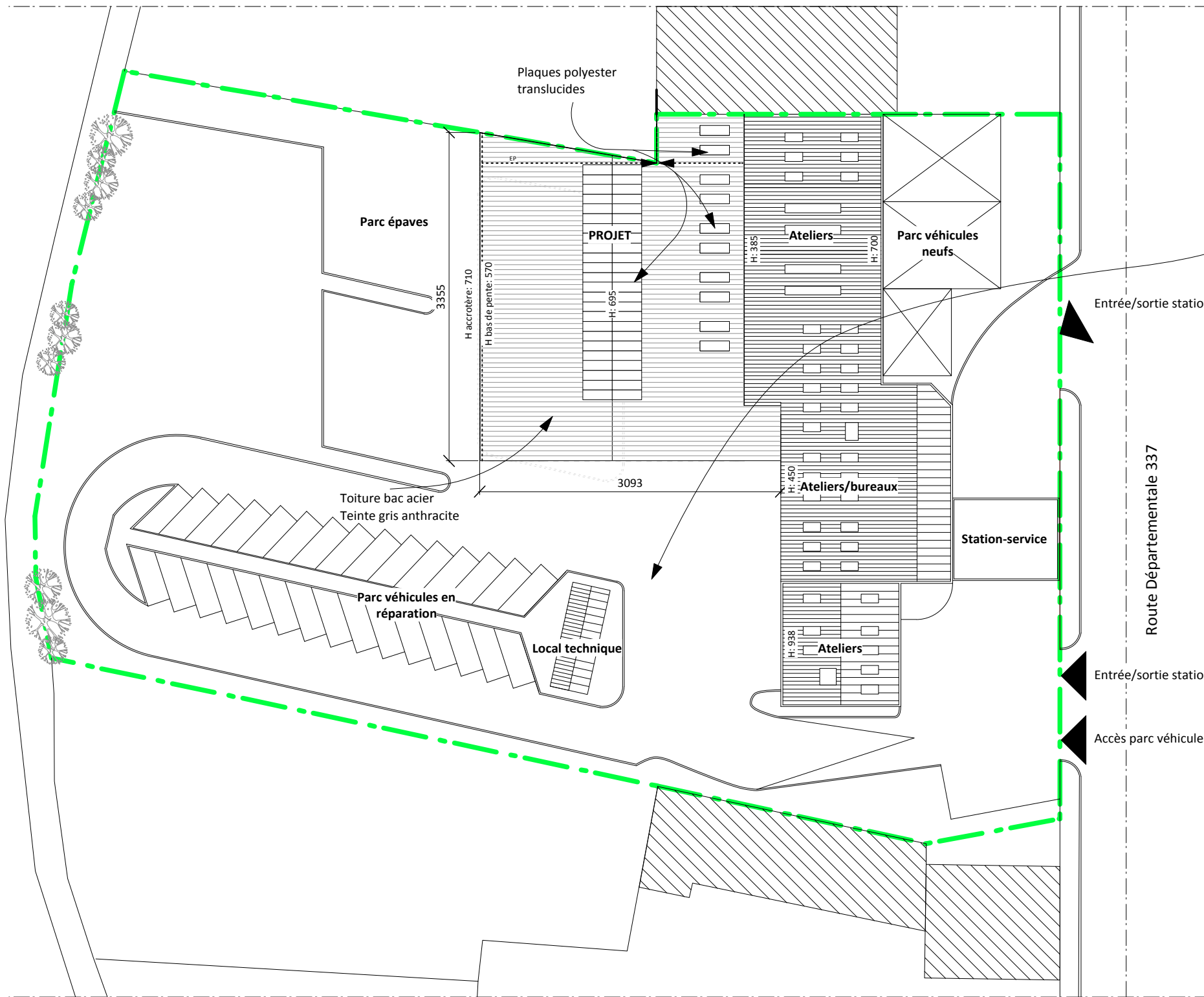
Plan-masse
