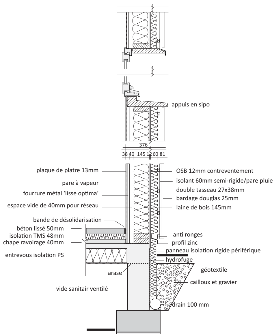
detail 1-1:20
