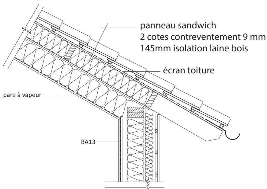
detail 2-1:20
