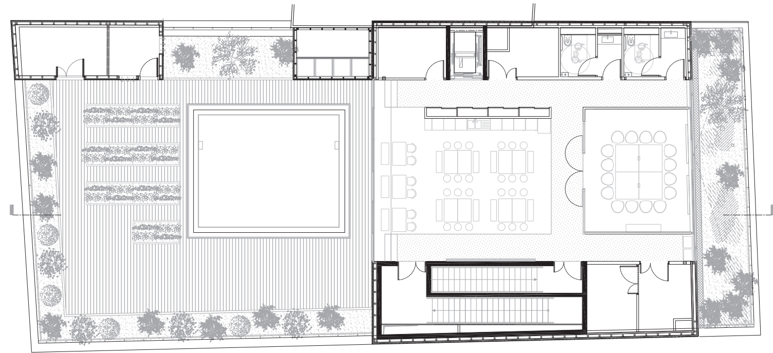
R+3 0 1 2 3 4 5m
